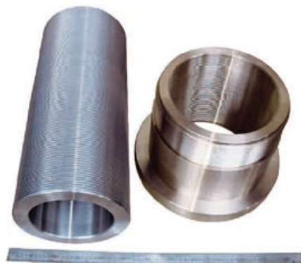
S45C (H) φ230×540 (TM230×P5) PBC φ355×245 (TM230×P5)
